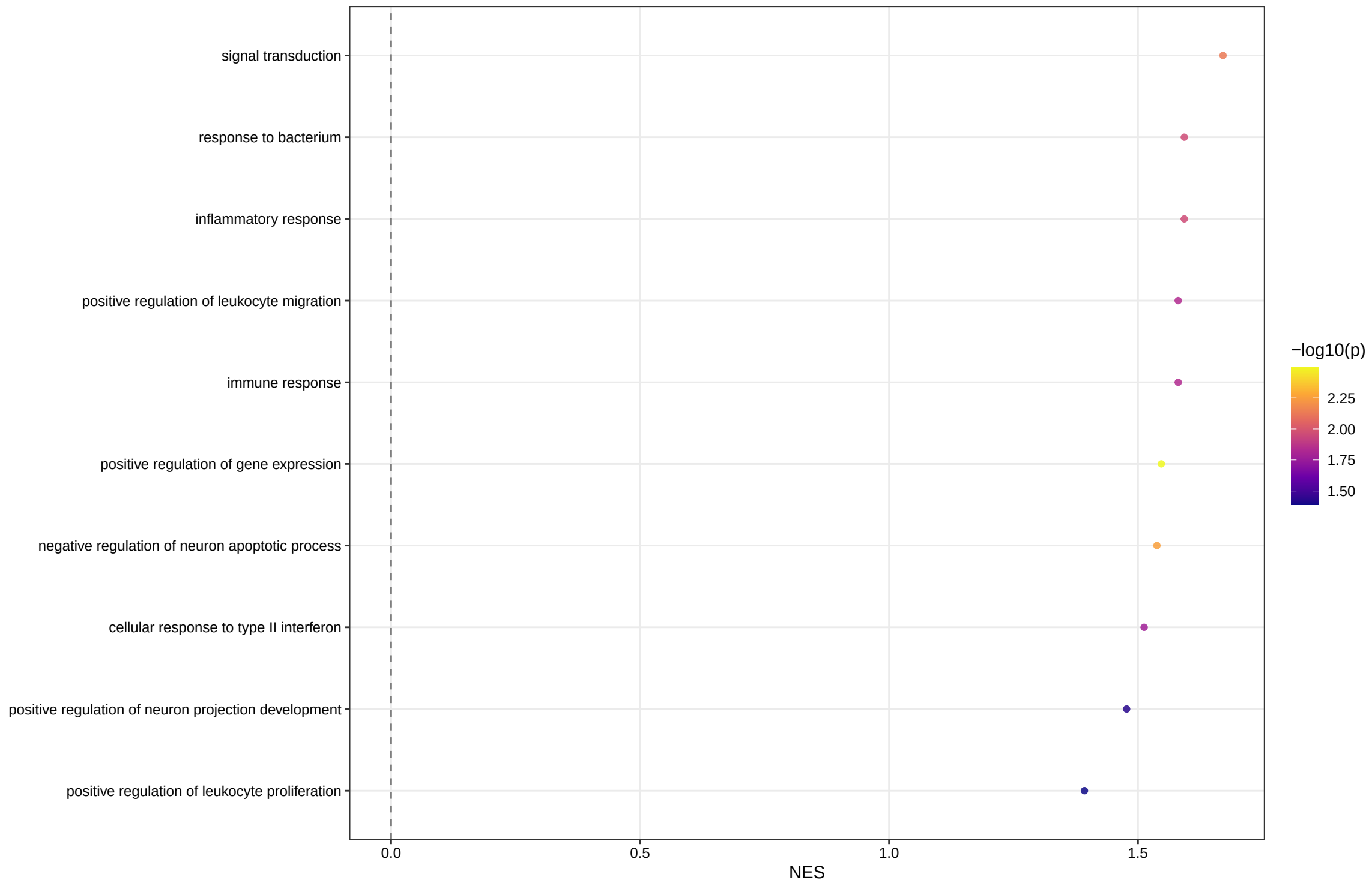
GO:BP GSEA – Nuclear factor 1
