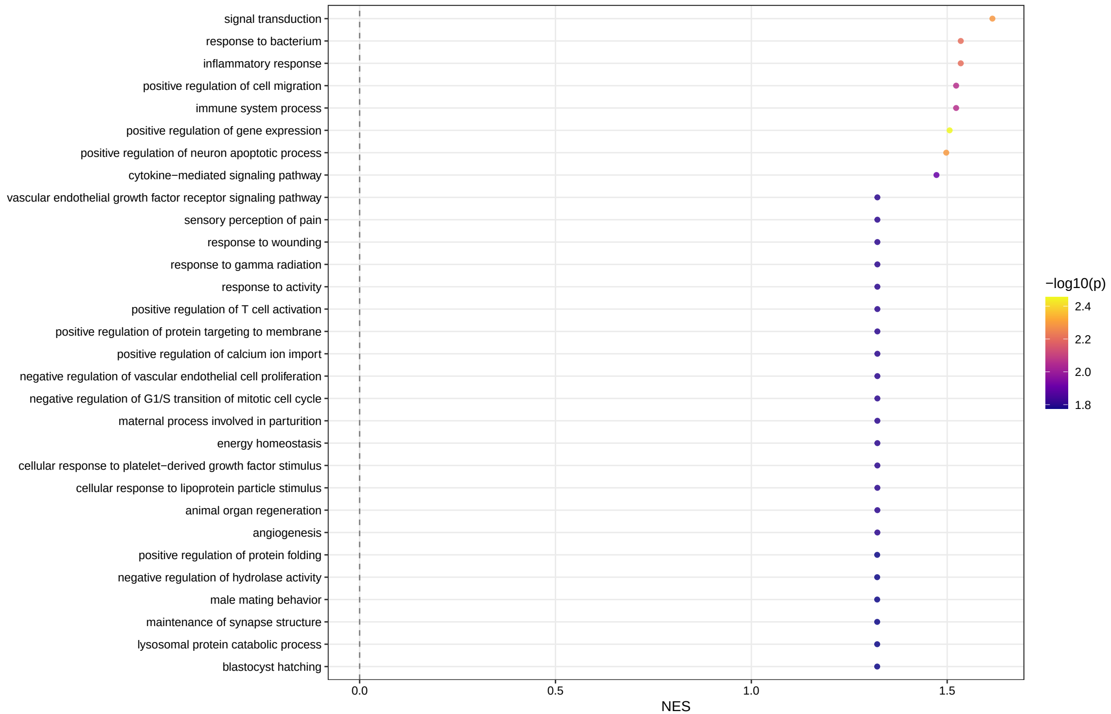
GO:BP fgsea – Nuclear factor 1
